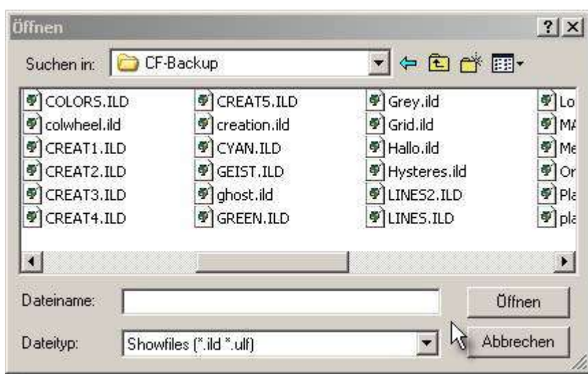
Fig.6 Filedialog
