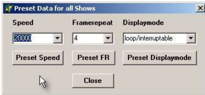
Fig.9 Preset Button
