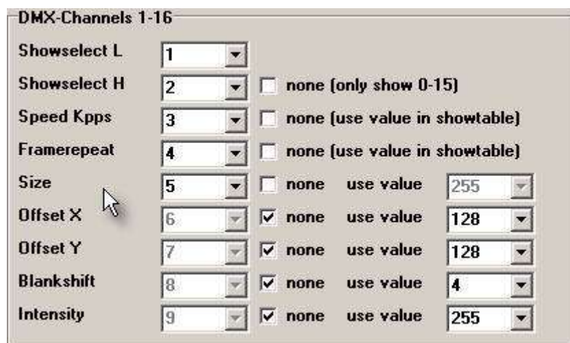
Fig. 4 DMX-channel selection
