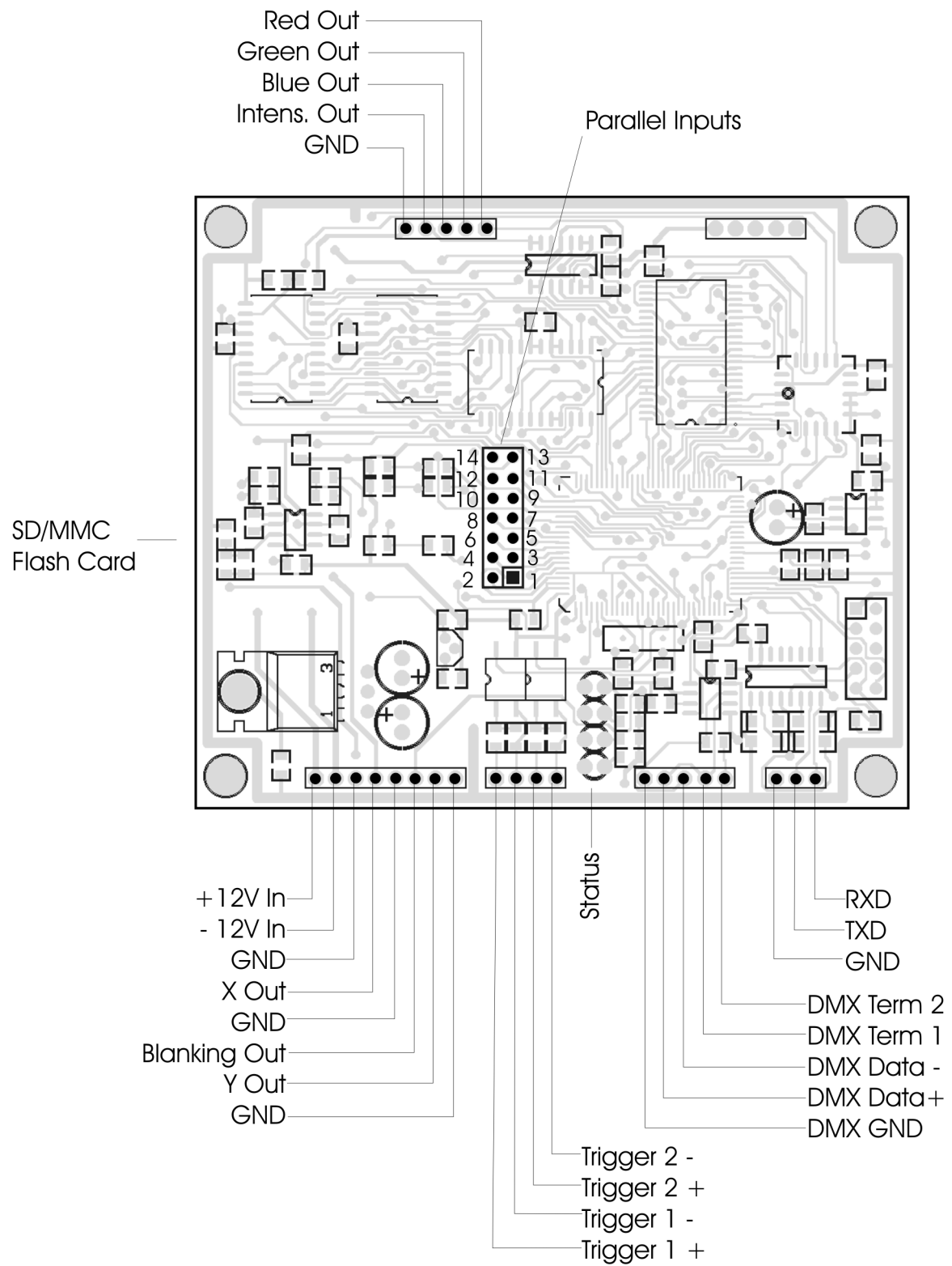
Fig. 1 Boardlayout
